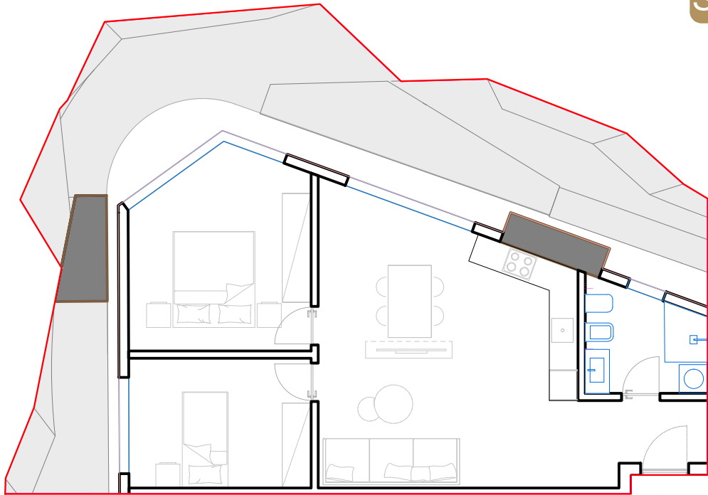
Plan mobilimi
