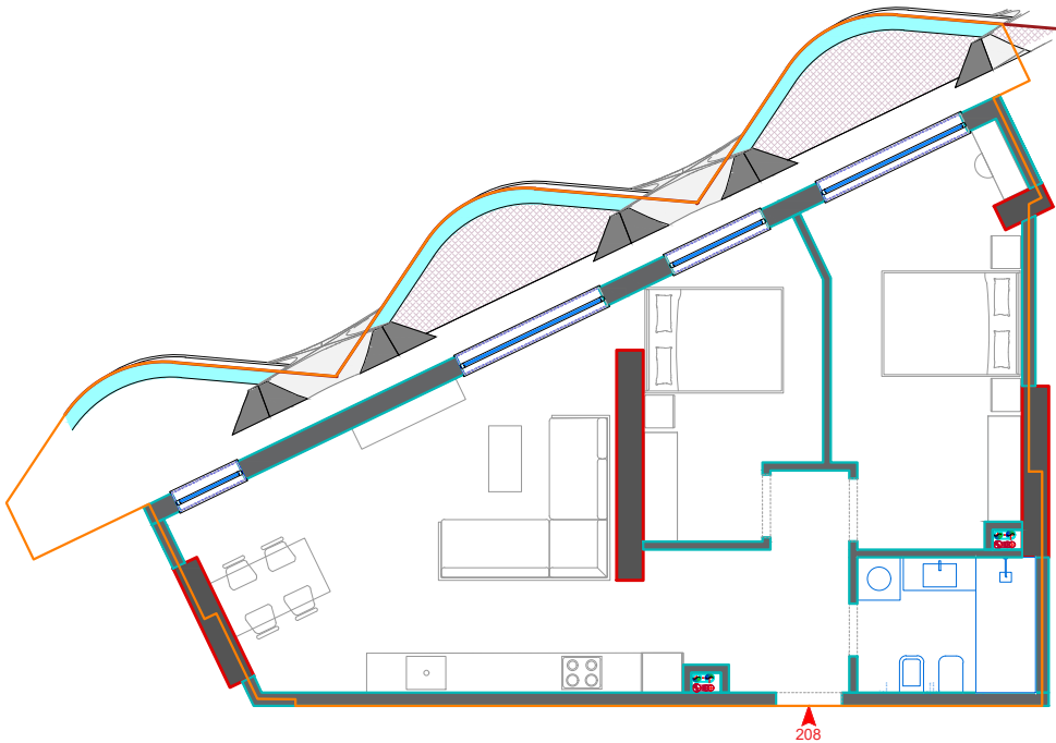
Plan Mobilimi
